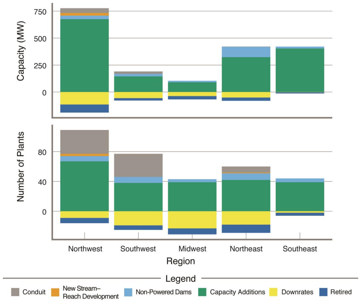
Figure 6. Recent hydropower capacity changes by region and project type (2005–2013)
